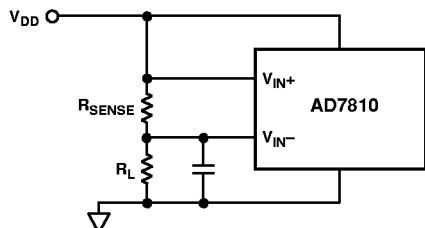
Figure 9. DC Current Measurement Scheme
