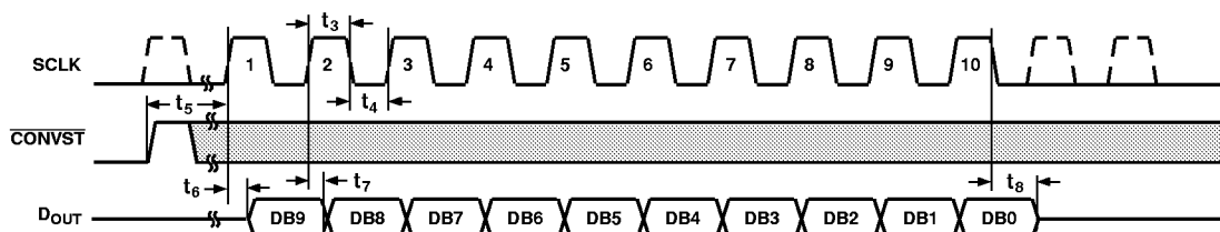
Figure 16. AD7810 Serial Interface Timing
