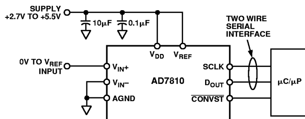
Figure 6. Typical Connection Diagram
