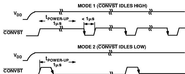
Figure 12. Power-Up Times
