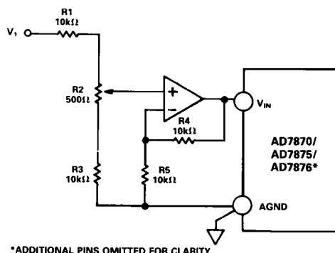
Figure 8. Offset and Full-Scale Adjust Circuit
