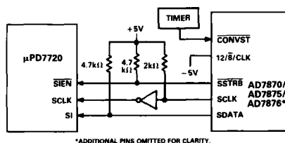
Figure 22. NEC7720 Serial Interface
