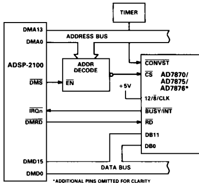
Figure 17. ADSP-2100 Parallel Interface
