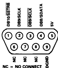
Figure 27. SKT5, D-Type Connector Pinout
