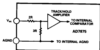
Figure 5c. AD7875 Analog Input
