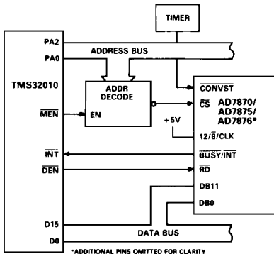
Figure 18. TMS32010 Parallel Interface
