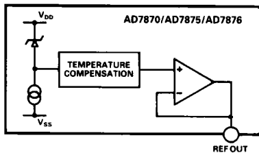
Figure 3. Reference Circuit
