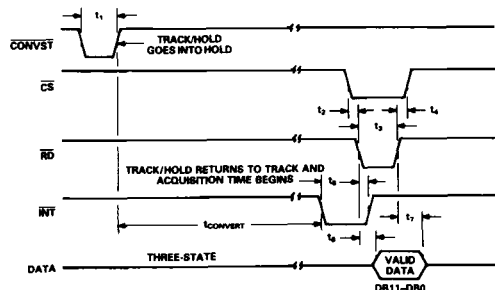
Figure 9. Mode 1 Timing Diagram, 12-Bit Parallel Read
