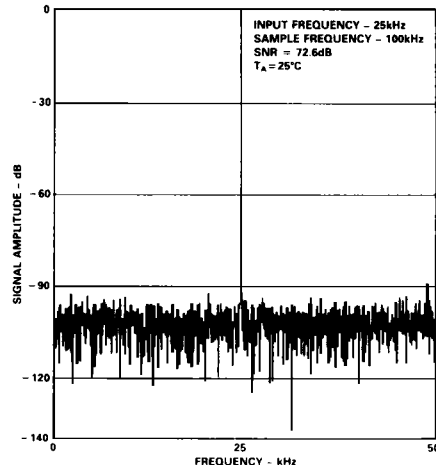
Figure 13. FFT Plot
