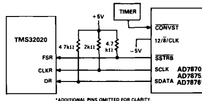
Figure 23. TMS32020 Serial Interface
