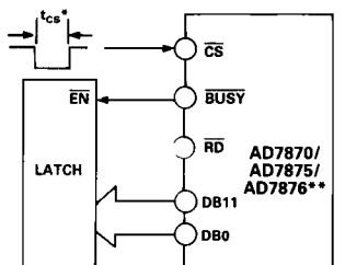
Figure 25. Stand-Alone Operation
