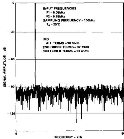
Figure 15. IMD Plot
