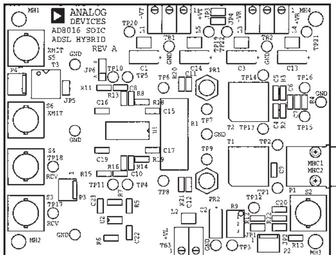
Figure 47. Assembly
