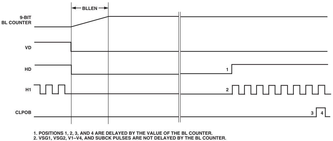
Figure 25. VD, HD, and H1 Extended Blanking Operation HBLKEXT = 1
