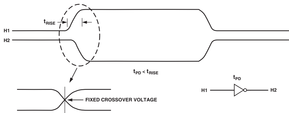
Figure 14. H-Clock Inverse Phase Relationship
