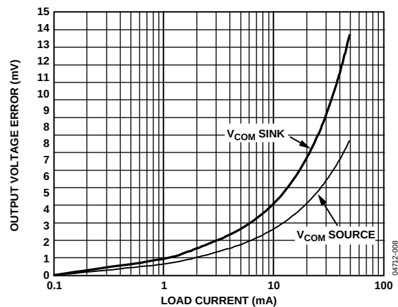
Figure 8. Output Voltage Error vs. Load Current ( V_{COM} )
