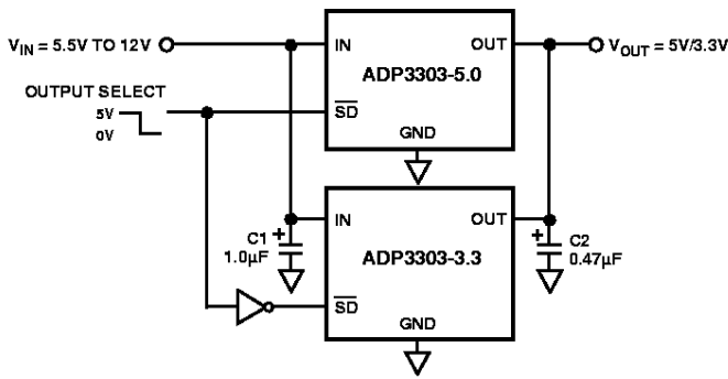
Figure 23. Crossover Switch
