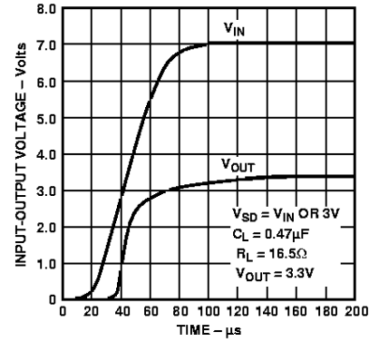
Figure 10. Power-Up Transient
