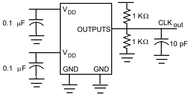
Figure 8. Test Circuit 2
