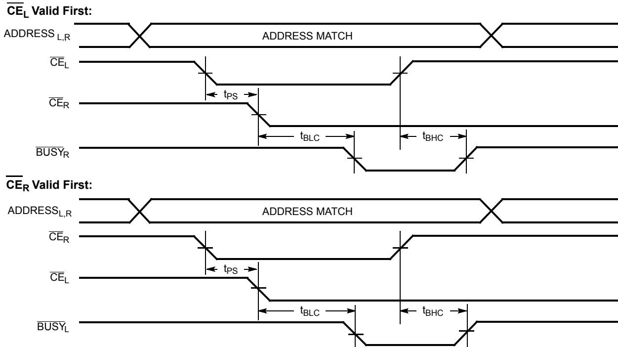
Figure 8. Busy Timing Diagram No. 1 ( \overline{CE} Arbitration)
