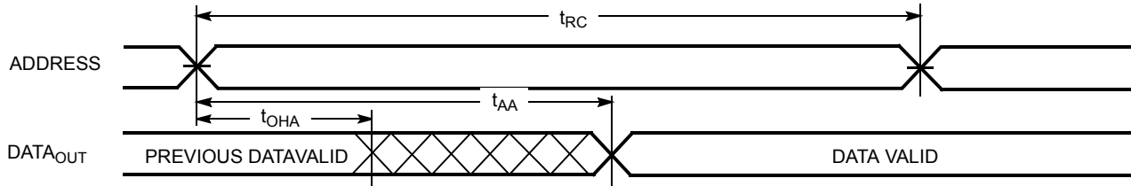
Figure 4. Read Cycle No. 2 [19, 21]
