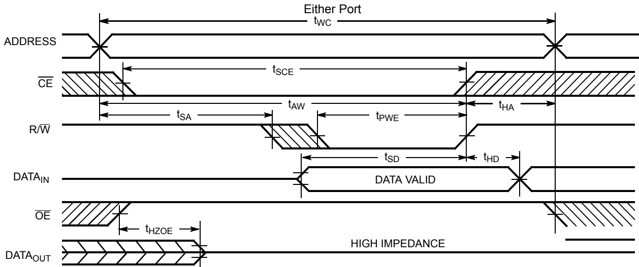
Figure 7. Write Cycle No. 2 ( \overline{R/\overline{W}} Three-States Data I/Os – Either Port) [24, 25]
