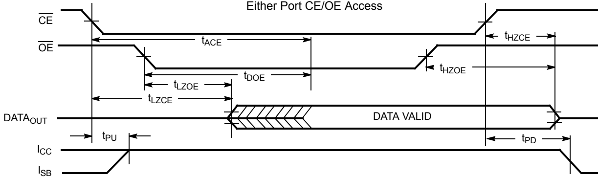
Figure 5. Read Cycle No. 3 [20]
