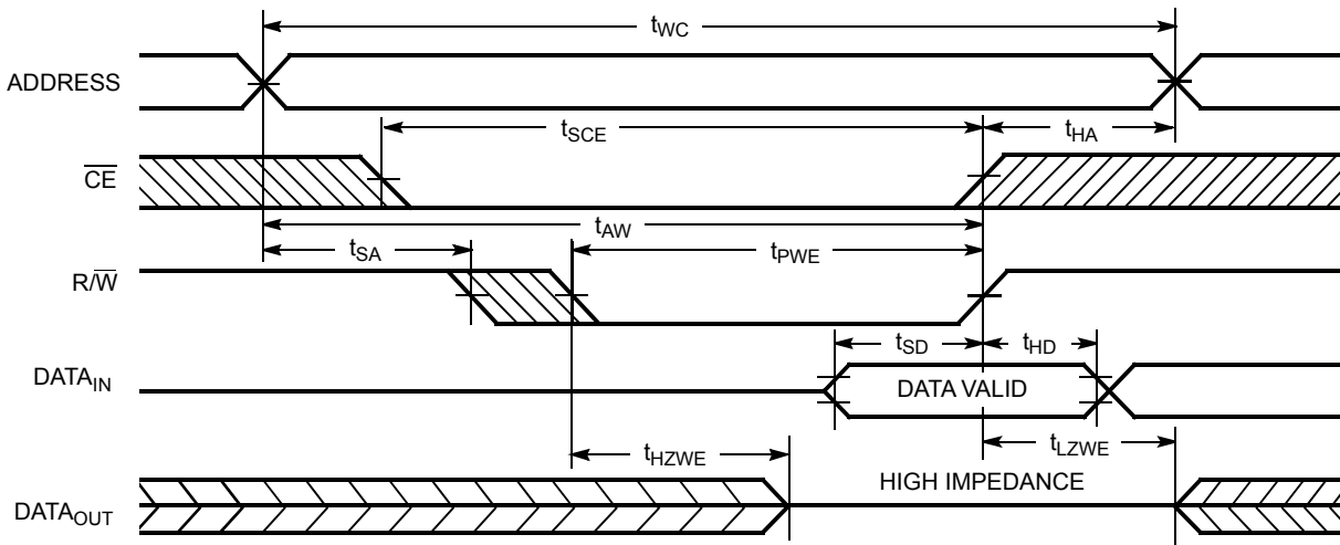
Figure 7. Write Cycle No. 2 ( \overline{R/\overline{W}} Three-States Data I/Os – Either Port) [24, 25]
