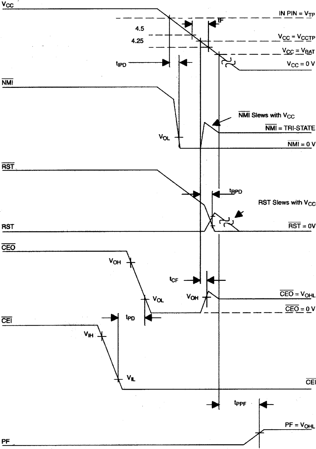
POWER-DOWN TIMING Figure 10
