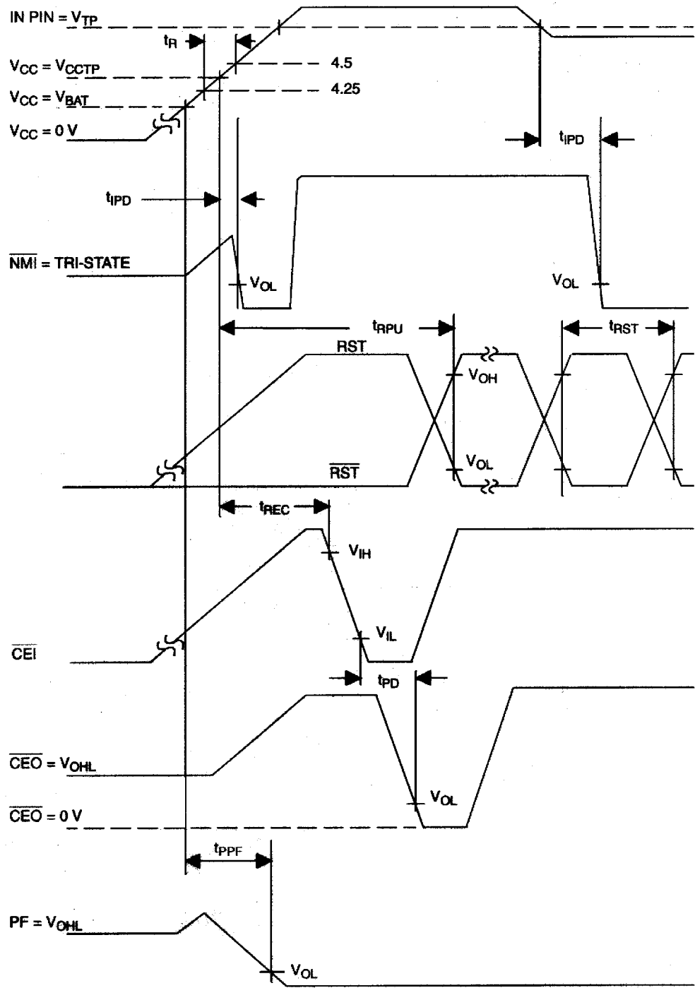
POWER-UP TIMING Figure 11
