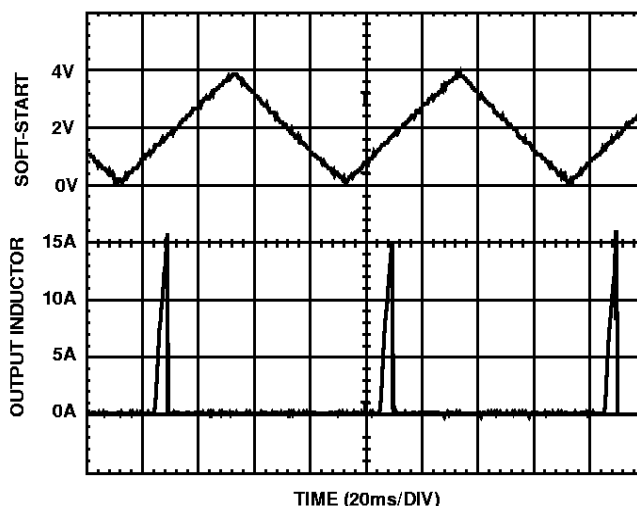
FIGURE 4. OVER-CURRENT OPERATION
