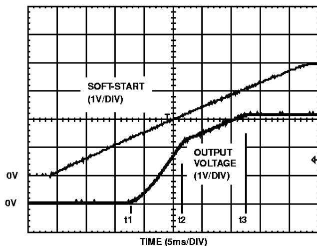
FIGURE 3. SOFT-START INTERVAL
