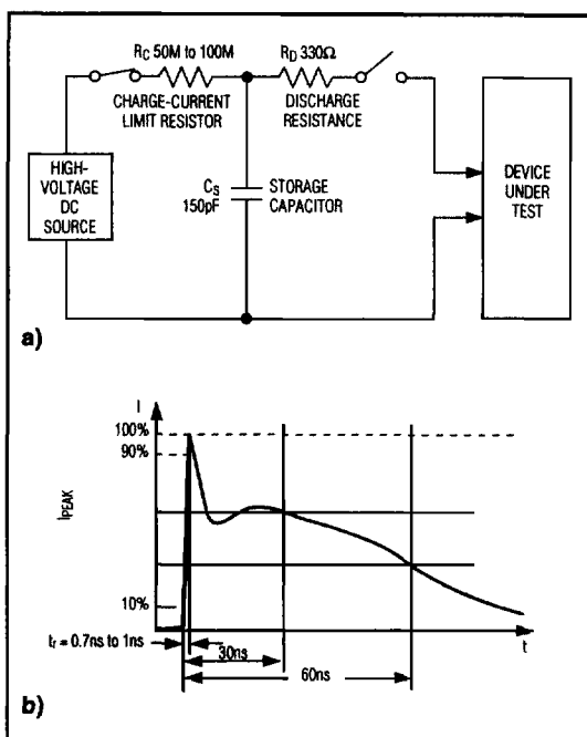
Figure 3. IEC1000-4-2 Test Model and ESD-Generator Current Waveform
