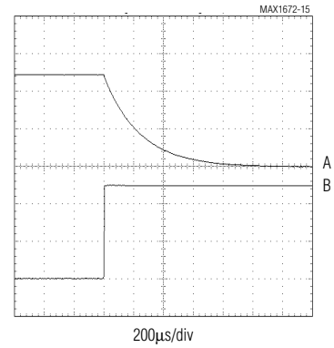
TURN-OFF DELAY
