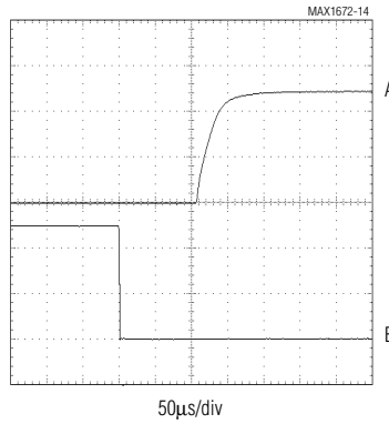
STARTUP DELAY
