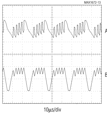
OUTPUT RIPPLE (HEAVY LOAD)
