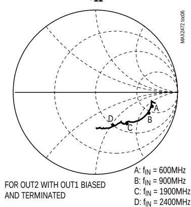
S_{11}
