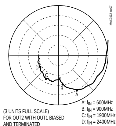
S_{21}
