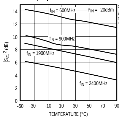
|S_{21}|^2 vs. TEMPERATURE
