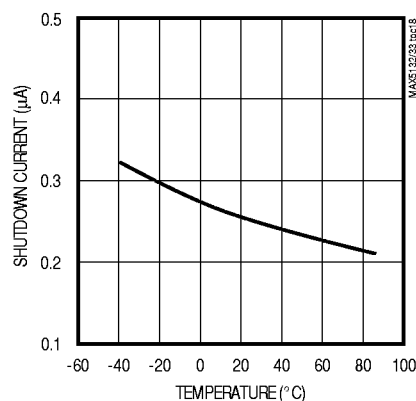
MAX5133 SHUTDOWN CURRENT vs. TEMPERATURE
