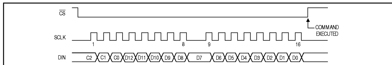
Figure 6. Serial-Interface Timing
