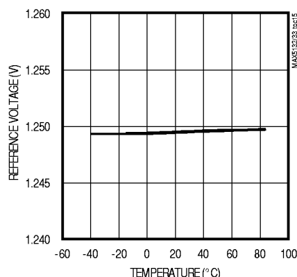
MAX5133 REFERENCE VOLTAGE vs. TEMPERATURE
