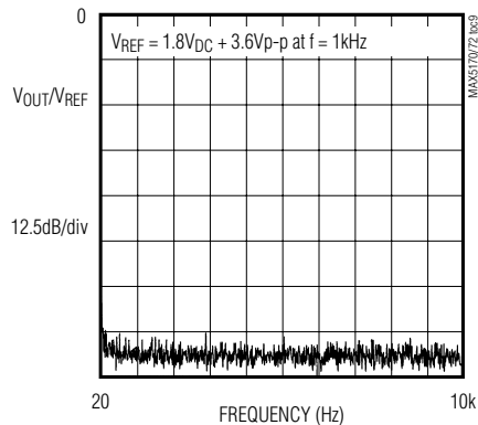
REFERENCE FEEDTHROUGH
