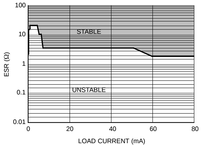
Figure 57. Ceramic Capacitor 2.2\text{ }\mu\text{F}
