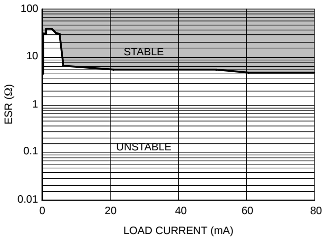
Figure 56. Ceramic Capacitor 1.0\text{ }\mu\text{F}
