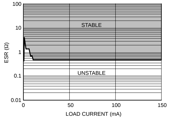
Figure 53. Ceramic Capacitor 2.2\text{ }\mu\text{F}
