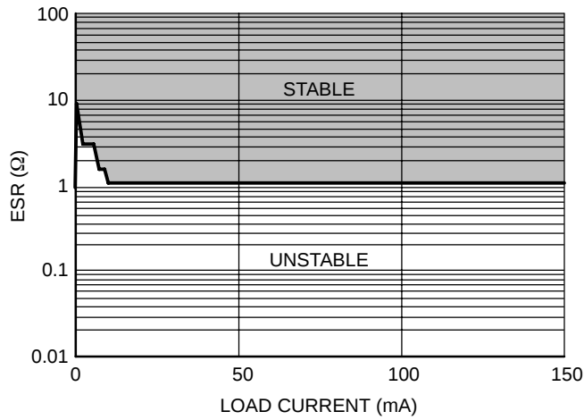
Figure 52. Ceramic Capacitor 1.0\text{ }\mu\text{F}
