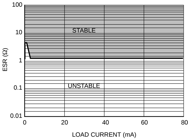
Figure 54. Ceramic Capacitor 1.0\text{ }\mu\text{F}
