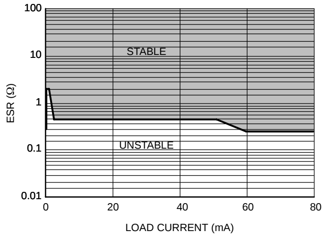
Figure 55. Ceramic Capacitor 2.2\text{ }\mu\text{F}
