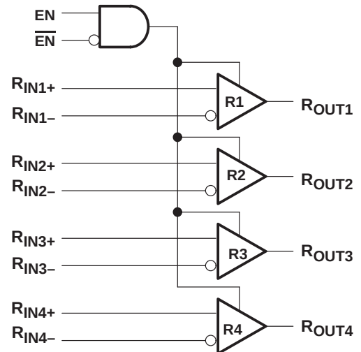
functional diagram
