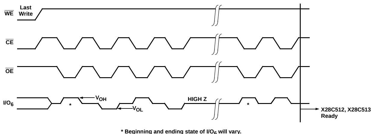
FIGURE 3A. TOGGLE BIT BUS SEQUENCE
