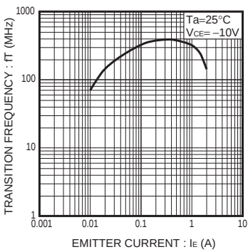
Fig.8 Transition Frequency
