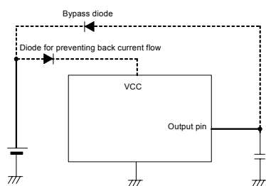
Fig.32 Bypass diode
