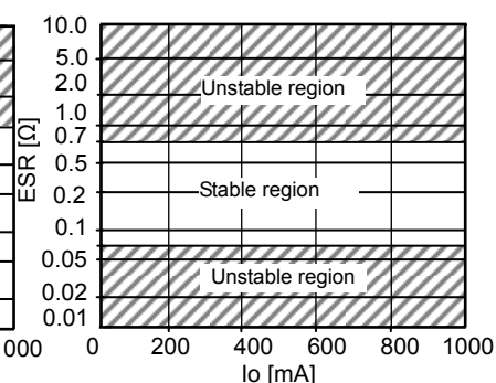
Fig.29 BA30E00WHFP ESR Characteristics
