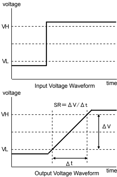
Fig. 230 Slew rate input output wave
