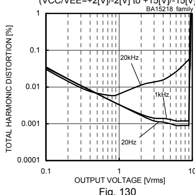
Fig. 130 Total Harmonic Distortion – Output Voltage ( V_{CC}/V_{EE}=+15[V]/-15[V] , A_v=20[dB] , R_L=2[k\Omega] , 80[kHz] -LPF, T_a=25[^\circ C] )
