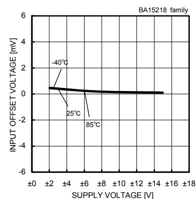
Input Offset Voltage - Supply Voltage (Vcm=0[V], Vout=0[V])
