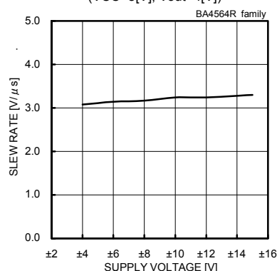
Fig. 106 Slew Rate - Supply Voltage ( C_L=100[pF] , R_L=2[k\Omega] , T_a=25[^\circ C] )
