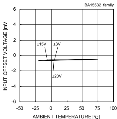
Fig. 252 Input Offset Voltage - Ambient Temperature (Vcm=0[V], Vout=0[V])
