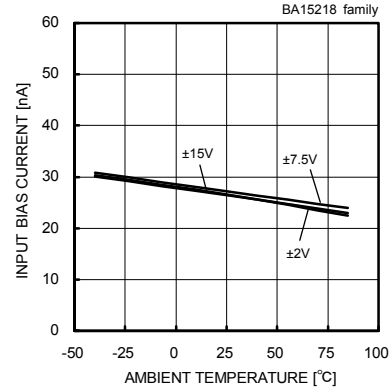
Input Bias Current - Ambient Temperature (Vcm=0[V], Vout=0[V])
