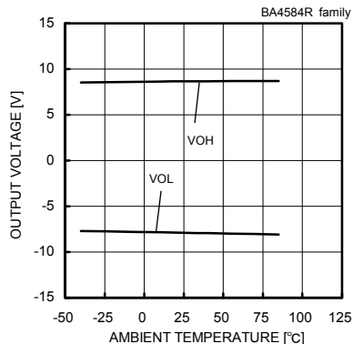
Fig. 161 Maximum Output Voltage - Ambient Temperature (VCC/VEE=±9.5[V]/-9.5[V], RL=2[kΩ])
