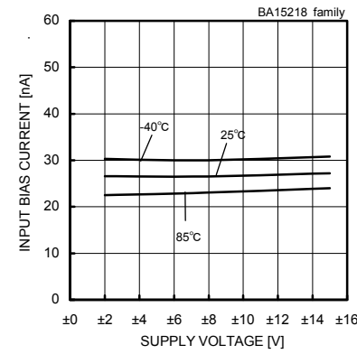
Input Bias Current - Supply Voltage (Vcm=0[V], Vout=0[V])
