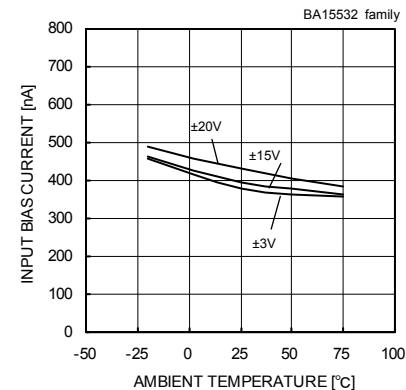
Fig. 254 Input Bias Current - Ambient Temperature (Vcm=0[V], Vout=0[V])
