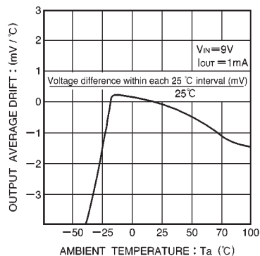
Fig.8 Output average drift within each 25°C
