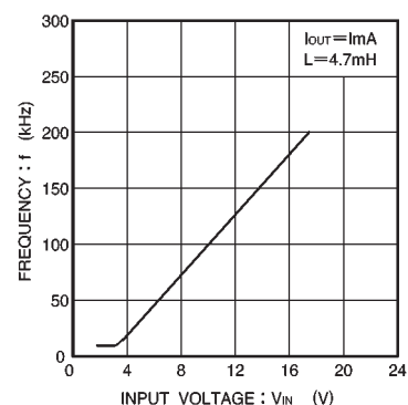
Fig.11 Oscillation frequency vs. input voltage
