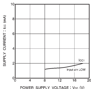
Fig.1 Current dissipation 1 vs. power supply voltage
