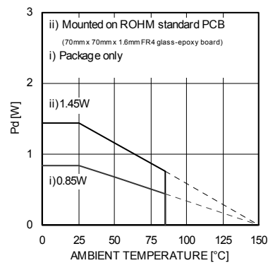
Fig.7 Thermal derating curve (BA6247FP-Y, HSOP25)
