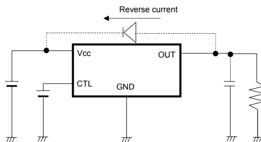
Fig.27 Bypass diode
