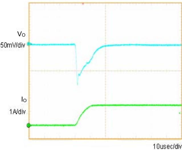
Fig.3 Transient Response (0→1.5A) Co=1μF
