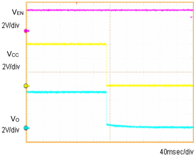
Fig.6 OFF sequence 1 Co=1μF
