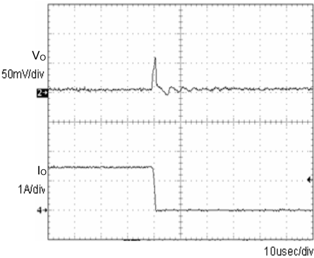
Fig.4 Transient Response (1.5→0A) Co=1μF
