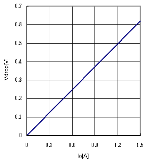
Fig.22 Minimum dropout Voltage 2 ( V_{cc}=4.5 V, T_a=25^{\circ}\text{C} )
