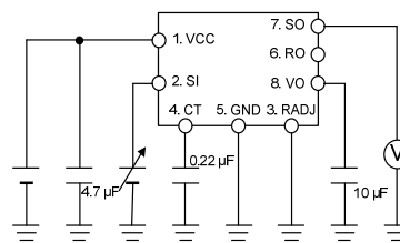
Measurement Circuit for Figure 17, 18
