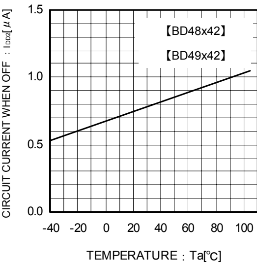
Fig.10 Circuit Current when OFF
