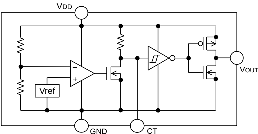
Figure.2 BD53Exxx-M Series
