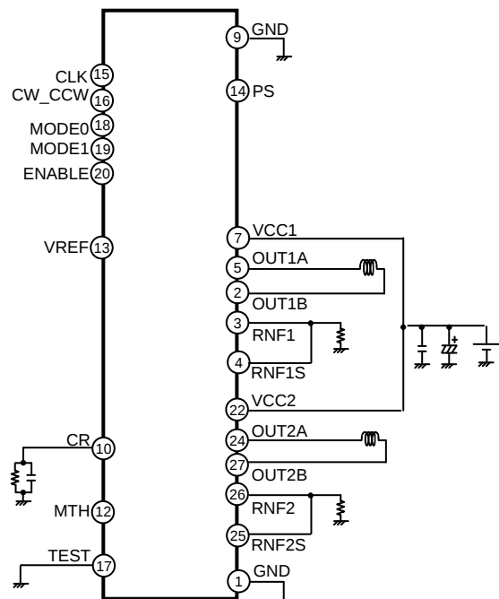
Figure.1 BD63715AEFV application circuit diagram
