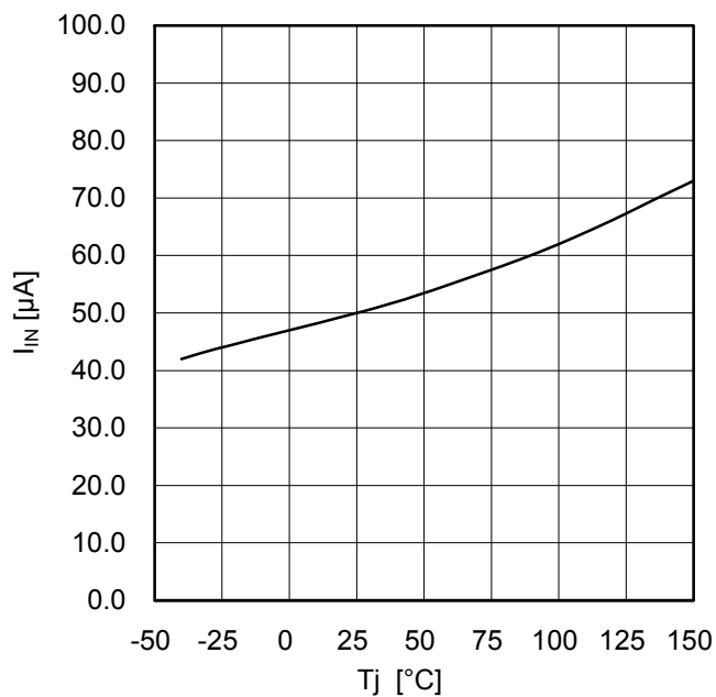
Figure 12. Input current Characteristic [Temperature Characteristic] (IN1 to 4, DIR, SCLK, SI, RST_B=5V, CS_B=0V)
