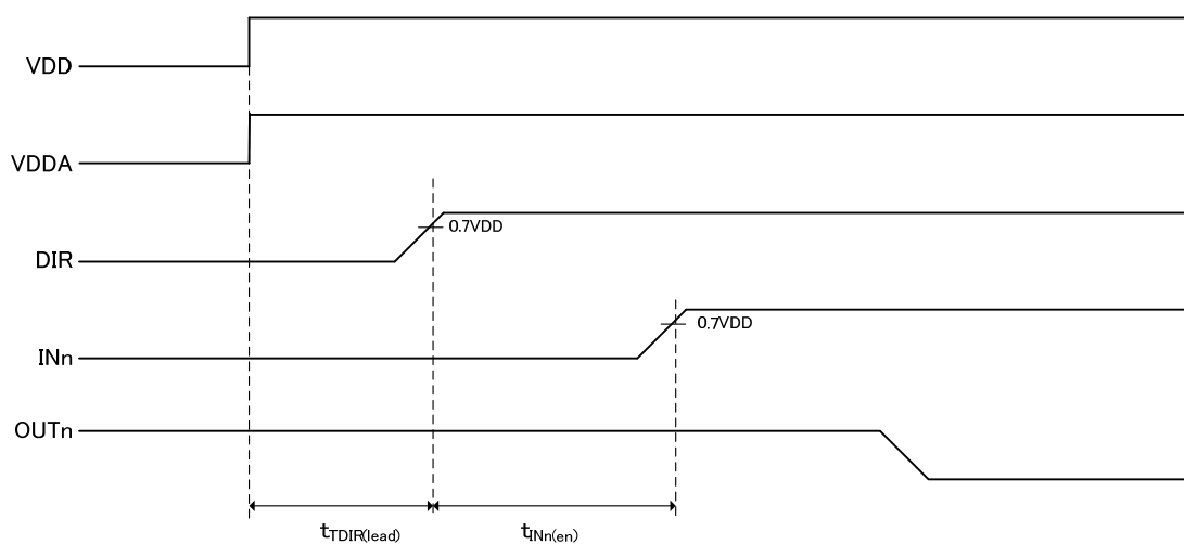
Figure 25. DIR Mode Timing Chart (1)
