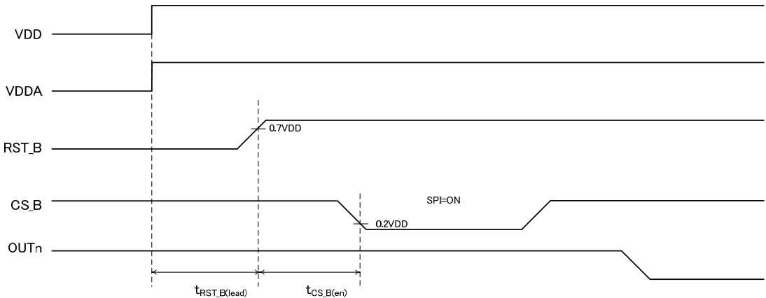
Figure 23. RST_B Releasing Sequence
