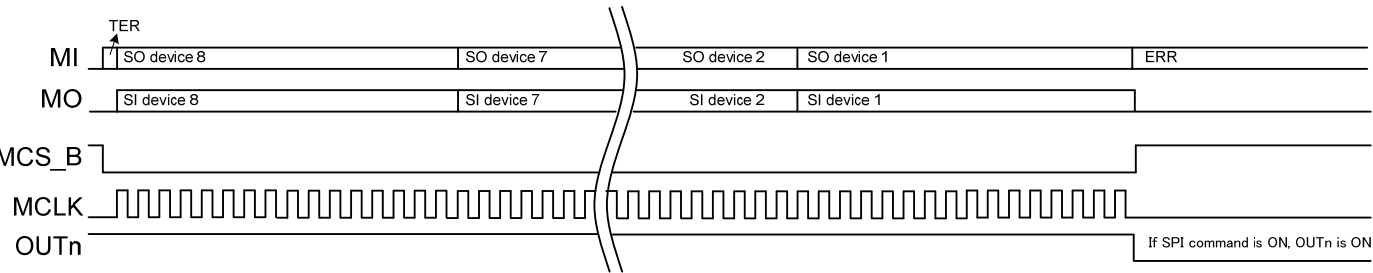
Figure 22. Timing chart when 8 devices are connected
