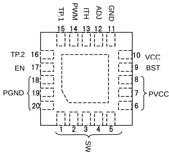
Fig.2 Pin configuration
