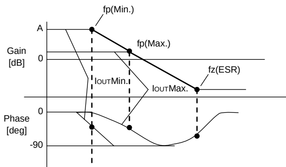
Fig.31 Open loop gain characteristics
