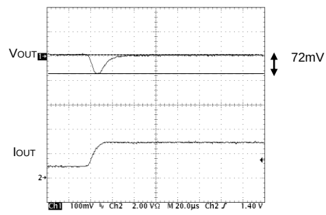
Fig.24 Comparison of transient response
