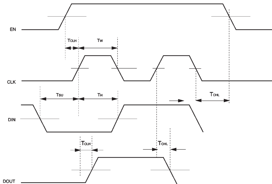
Fig. 2 Timing chart 1
