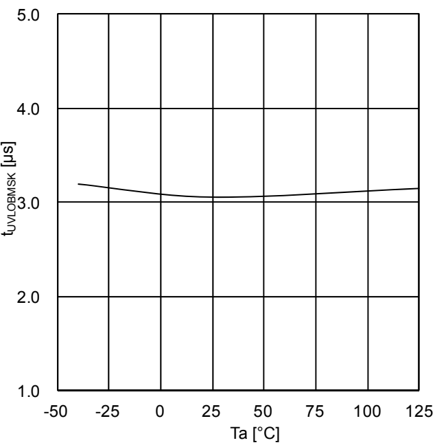
Figure 33. VCCB UVLOmask time
