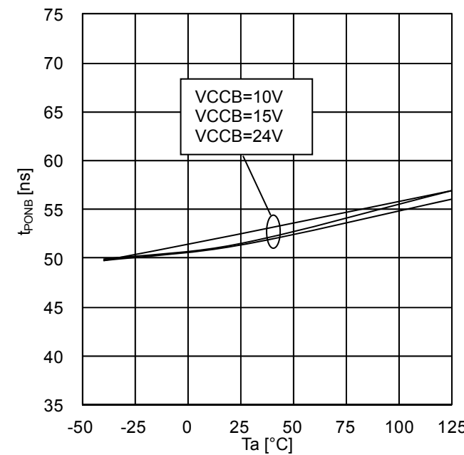
Figure 26. Turn ON Time (INA=L, INB=PWM)
