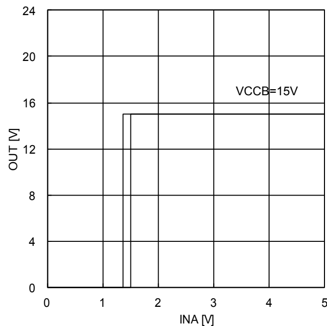
Figure 15. OUTA output voltage vs INA input voltage (VCCB=15V, VCCA=15V, Ta=25°C)
