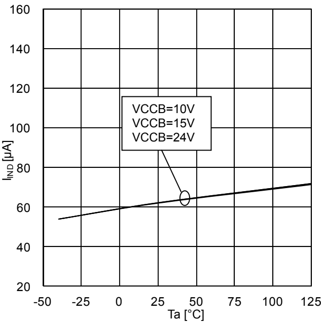
Figure 17. logic pull-down current
