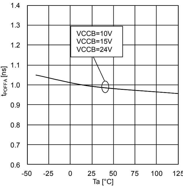
Figure 19. ENA input mask time
