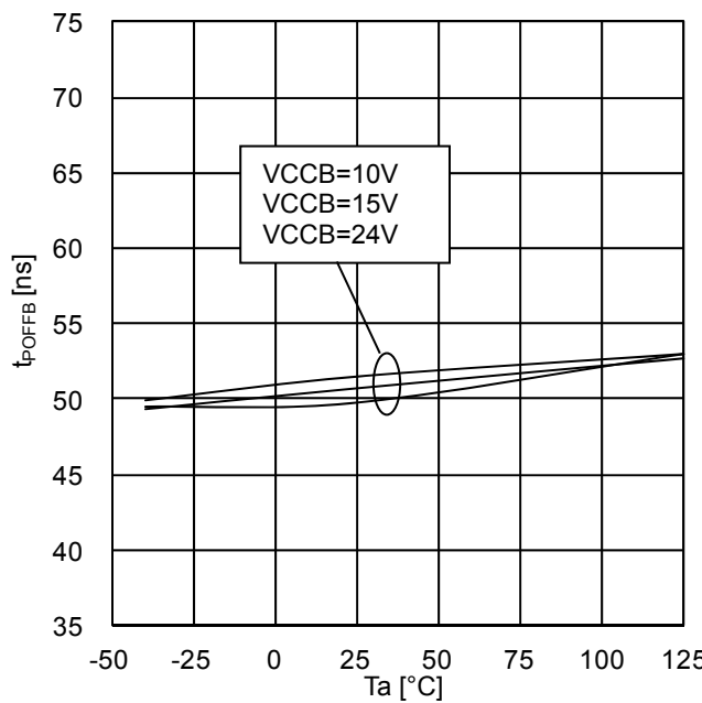
Figure 27. Turn OFF Time (INA=L, INB=PWM)
