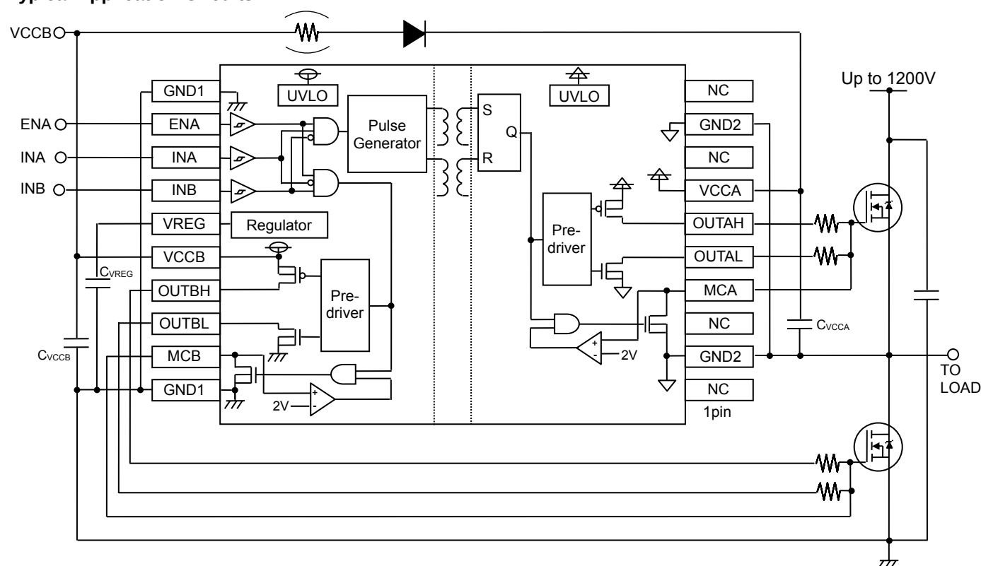
Figure 1. Typical Application Circuits
