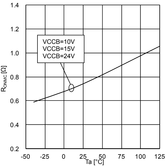
Figure 29. MCB ON resistance
