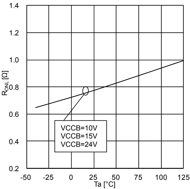
Figure 23. OUTB ON resistance (Sink)
