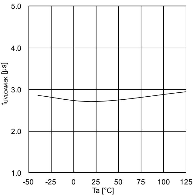
Figure 35. VCCA UVLO mask time
