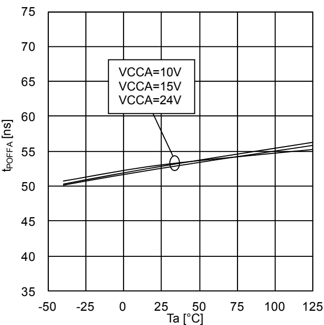
Figure 25. Turn OFF Time (INA=PWM, INB=L)
