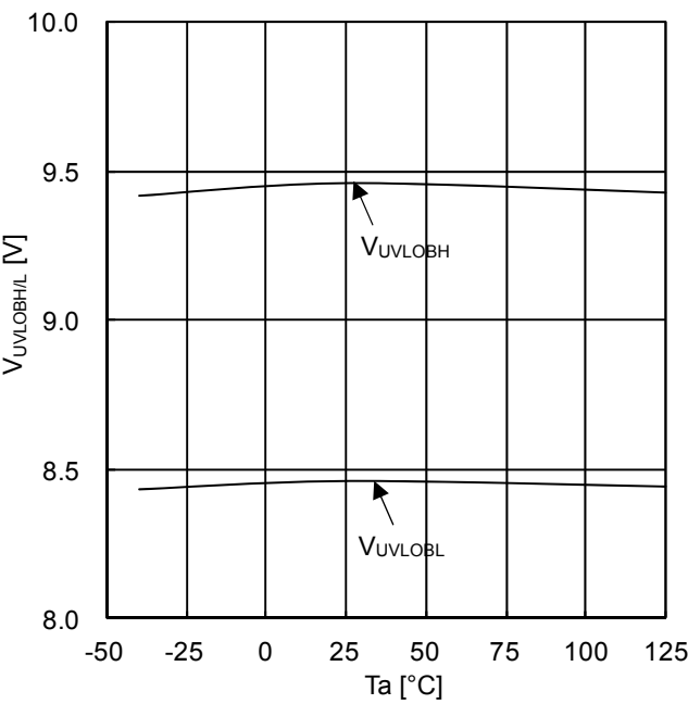
Figure 32. VCCB UVLO ON/OFF voltage
