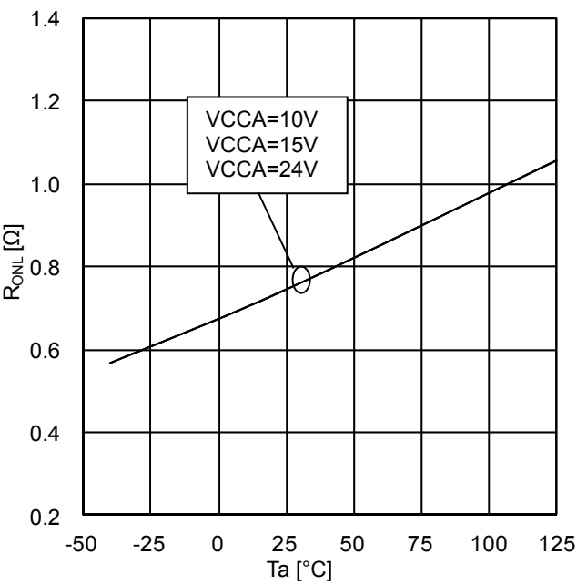
Figure 21. OUTA ON resistance (Sink)
