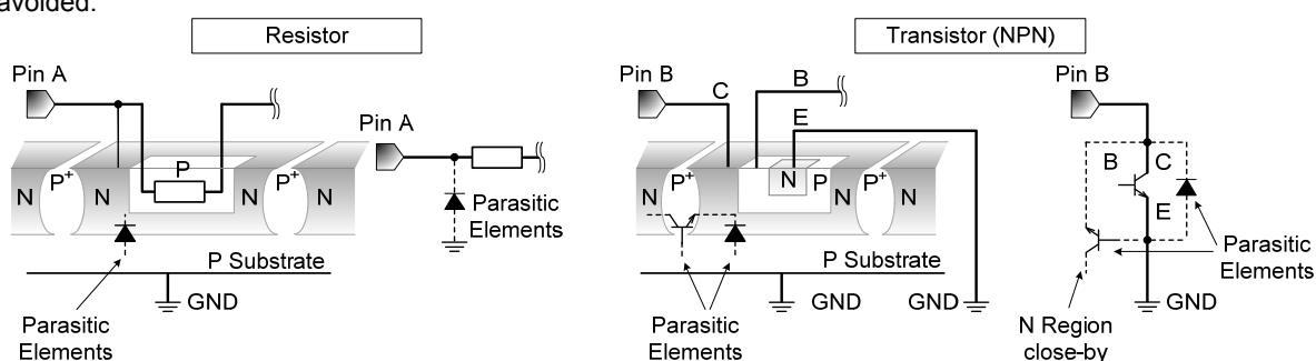
Figure 37. Example of IC structure
