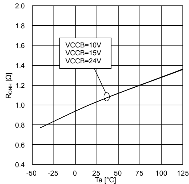
Figure 22. OUTB ON resistance (Source)
