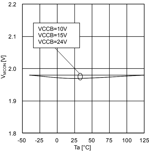
Figure 31. MCB ON threshold
