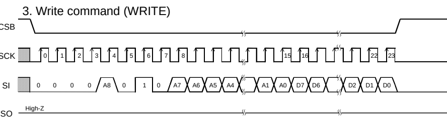
Figure 38. Write command
