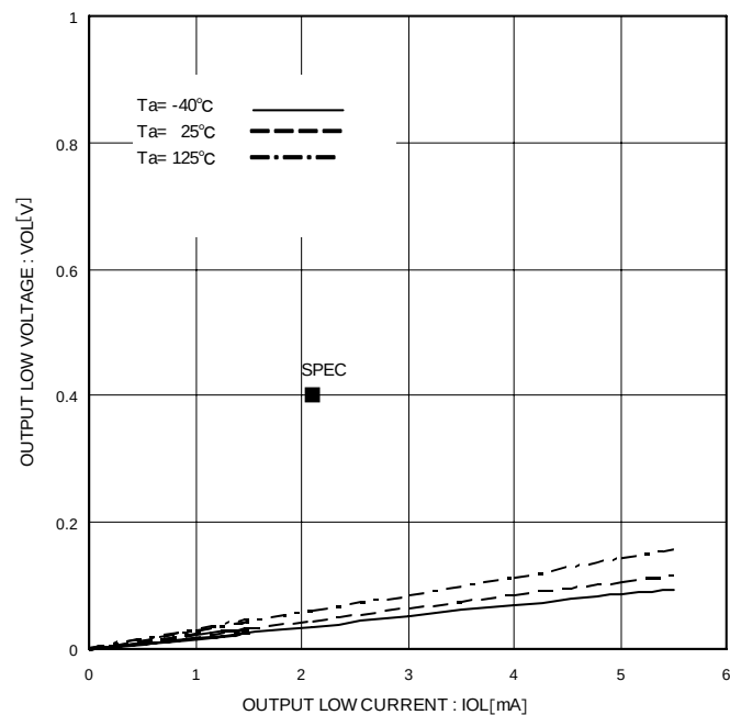
Figure 9. Output Low Voltage V_{OL} , I_{OL} ( V_{CC}=2.5\text{V} )
