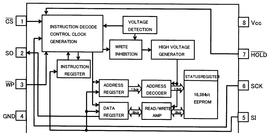
Fig.1 BLOCK DIAGRAM
