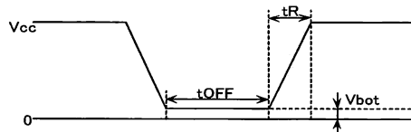
Fig.2 Vcc waveform
