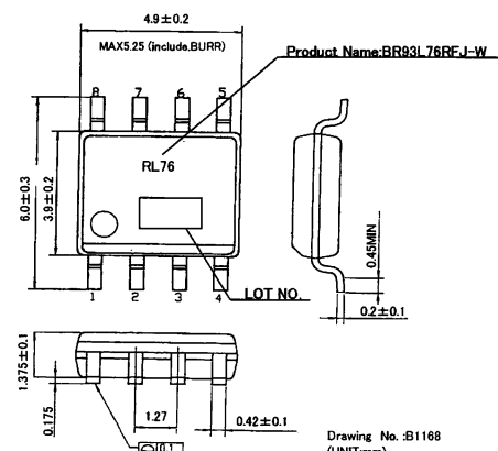
Fig.4-(f) PHYSICAL DIMENSION SOP-J8 (BR93L76RFJ-W)
