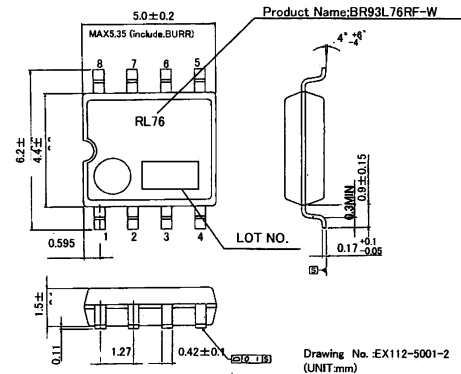
Fig.4-(d) PHYSICAL DIMENSION SOP8 (BR93L76RF-W)
