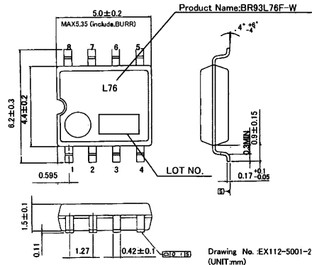
Fig.4-(c) PHYSICAL DIMENSION SOP8 (BR93L76F-W)
