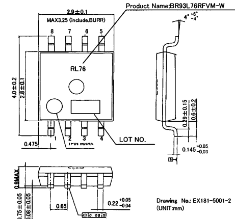
Fig.4-(b) PHYSICAL DIMENSION MSOP8 (BR93L76RFVW-W)
