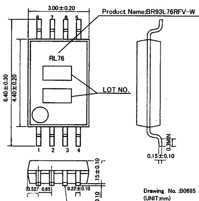
Fig.4-(h) PHYSICAL DIMENSION SSOP-B8 (BR93L76RFV-W)
