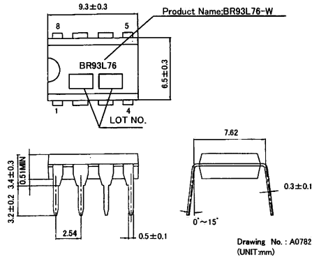
Fig.4-(a) PHYSICAL DIMENSION DIP8 (BR93L76-W)
