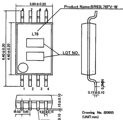
Fig.4-(g) PHYSICAL DIMENSION SSOP-B8 (BR93L76FV-W)
