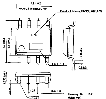
Fig.4-(e) PHYSICAL DIMENSION SOP-J8 (BR93L76FJ-W)
