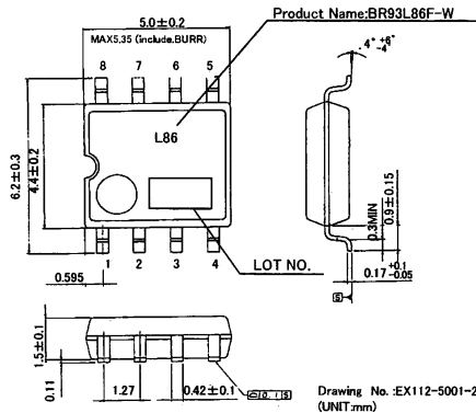
Fig.4-(c) PHYSICAL DIMENSION SOP8 (BR93L86F-W)
