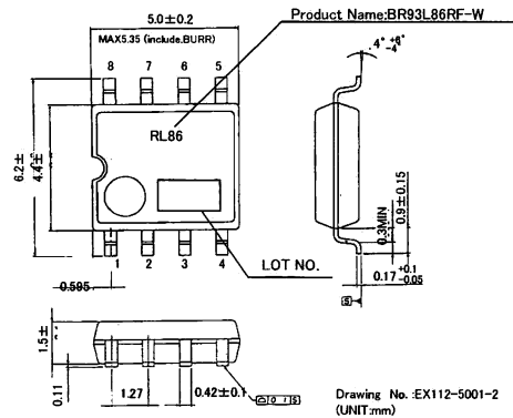
Fig.4-(d) PHYSICAL DIMENSION SOP8 (BR93L86RF-W)
