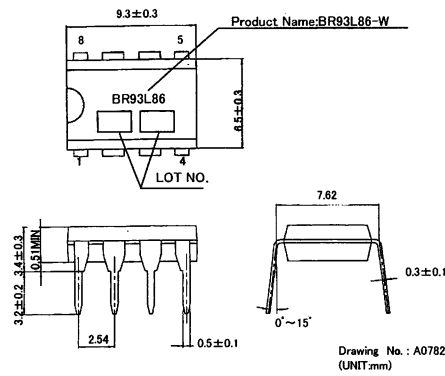
Fig.4-(a) PHYSICAL DIMENSION DIP8 (BR93L86-W)
