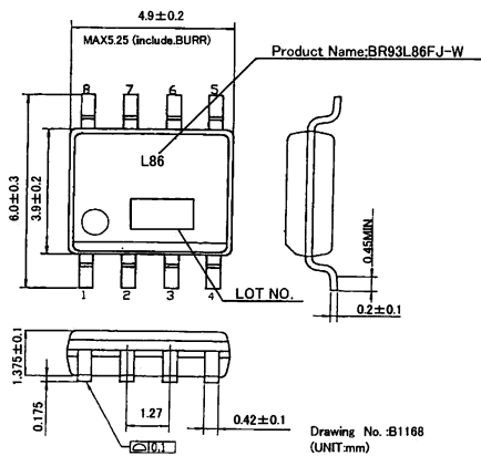
Fig.4-(e) PHYSICAL DIMENSION SOP-J8 (BR93L86FJ-W)
