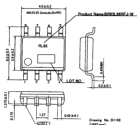
Fig.4-(f) PHYSICAL DIMENSION SOP-J8 (BR93L86RFJ-W)
