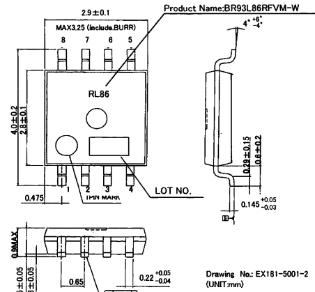
Fig.4-(b) PHYSICAL DIMENSION MSOP8 (BR93L86RFVM-W)
