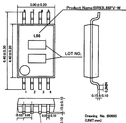
Fig.4-(g) PHYSICAL DIMENSION SSOP-B8 (BR93L86FV-W)
