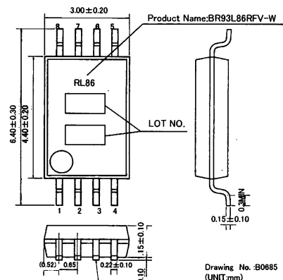
Fig.4-(h) PHYSICAL DIMENSION SSOP-B8 (BR93L86RFV-W)
