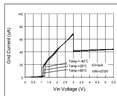
Fig. 123 Circuit Current IGND
