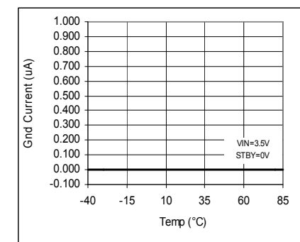
Fig. 16 IGND vs. Temp (STBY)
