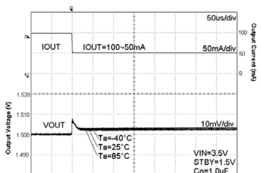
Fig. 23 Load Response
