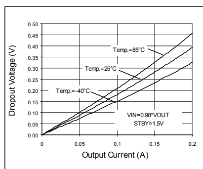
Fig. 66 Dropout Voltage
