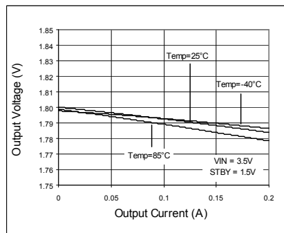
Fig. 40 Load Regulation
