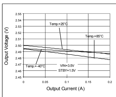
Fig. 69 Load Regulation
