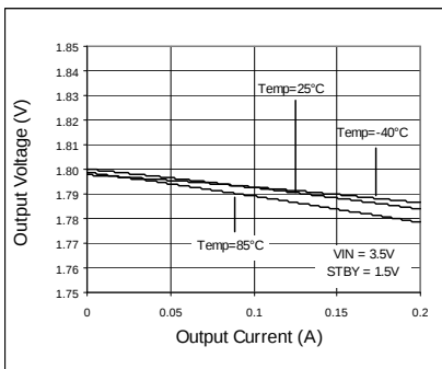
Fig. 40 Load Regulation
