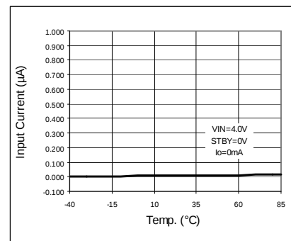
Fig. 132 IIGN vs Temp (STBY)
