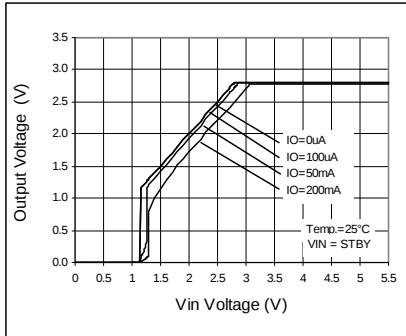
Fig. 92 Output Voltage
