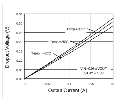
Fig. 153 Dropout Voltage
