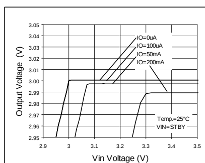
Fig. 122 Line Regulation
