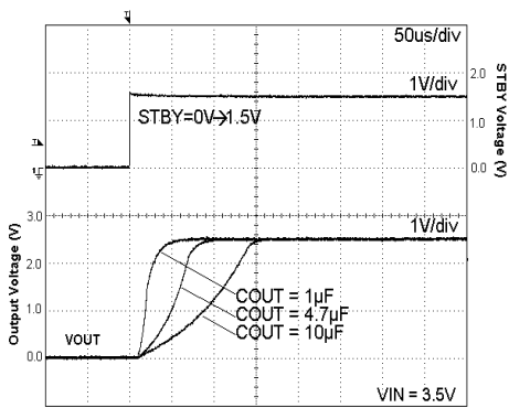
Fig. 86 Start Up Time I_{out} = 0\text{mA}
