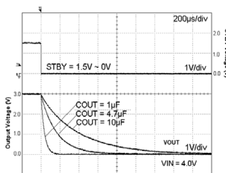
Fig. 148 Discharge Time I_{out} = 0\text{mA}
