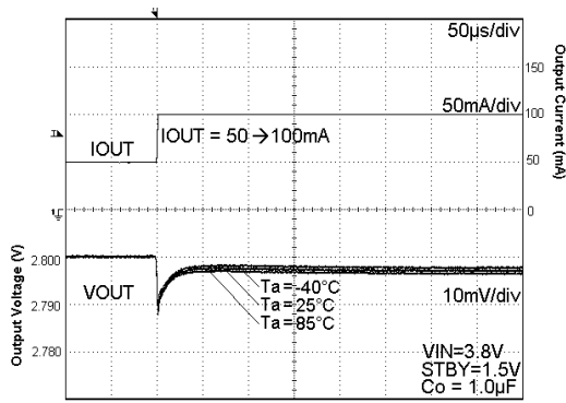
Fig. 109 Load Response
