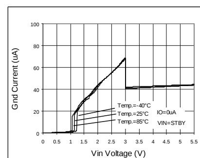
Fig. 123 Circuit Current IGND
