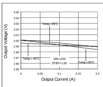
Fig. 127 Load Regulation
