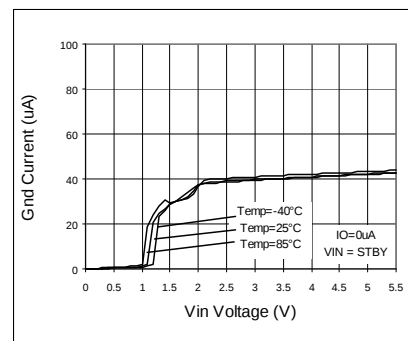
Fig. 7 Circuit Current IGND
