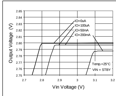
Fig. 93 Line Regulation
