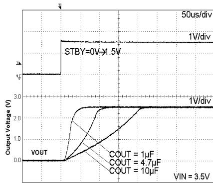
Fig. 87 Start Up Time I_{out} = 200\text{mA}
