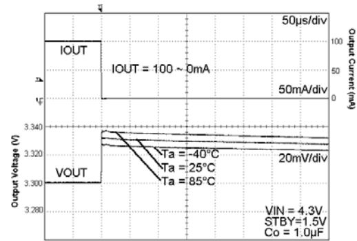
Fig. 166 Load Response
