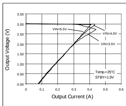
Fig. 128 OCP Threshold
