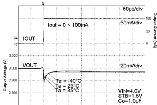
Fig. 136 Load Response
