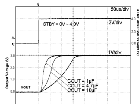
Fig. 146 Start Up Time (STBY=VIN) I_{out} = 0\text{mA}
