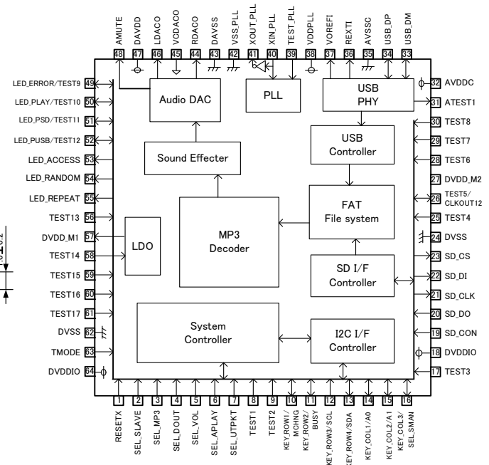
Figure 2. Block diagram
