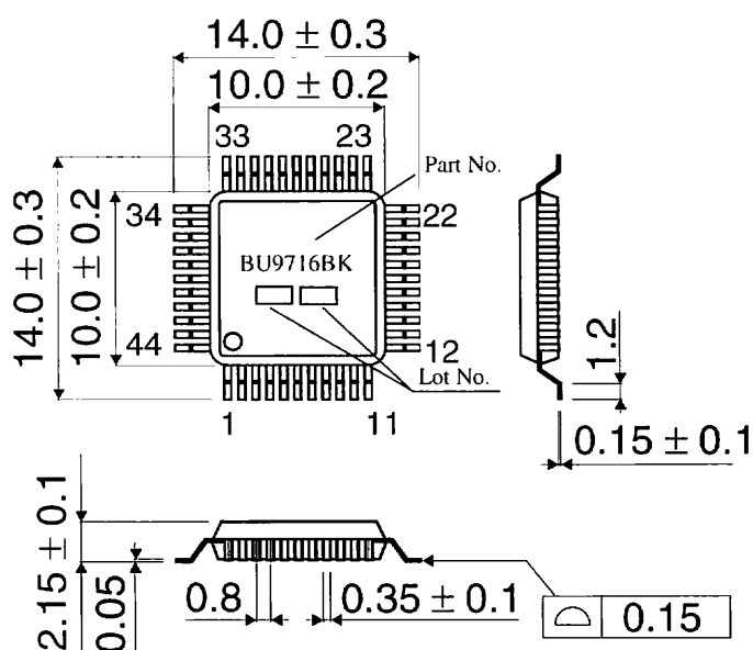
QFP-44 (Unit: mm)
