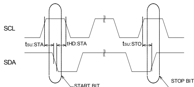
Fig.3 Synchronous Data Timing
