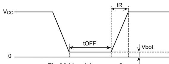
Fig.33 V CC rising wave from 0
