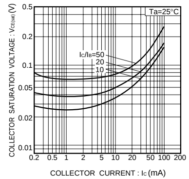
Fig.15 Collector-emitter saturation voltage vs. collector current
