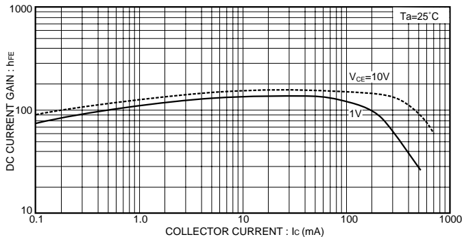
Fig.3 DC current gain vs. collector current (1)
