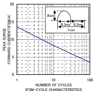
IFSM-CYCLE CHARACTERISTICS
