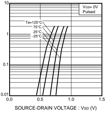
Fig.6 Source Current vs. Source-Drain Voltage
