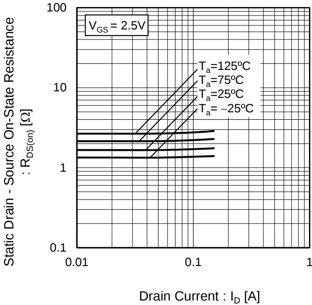
Fig.13 Static Drain-Source On-State Resistance vs. Drain Current(III)
